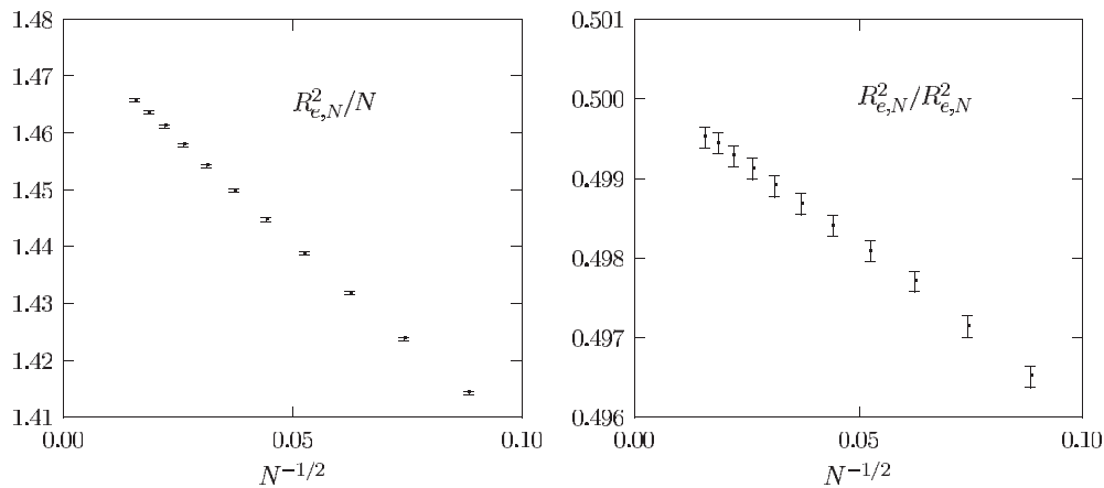
Figure 1. R_{e,N}^2/N and B_N = R_{m,N}^2/R_{e,N}^2 versus N^{-1/2} for d = 5 , showing clearly the presence of the N^{-1/2} -correction to scaling. From the right-hand side plot we extrapolate B_\infty = 0.5001(6) .
