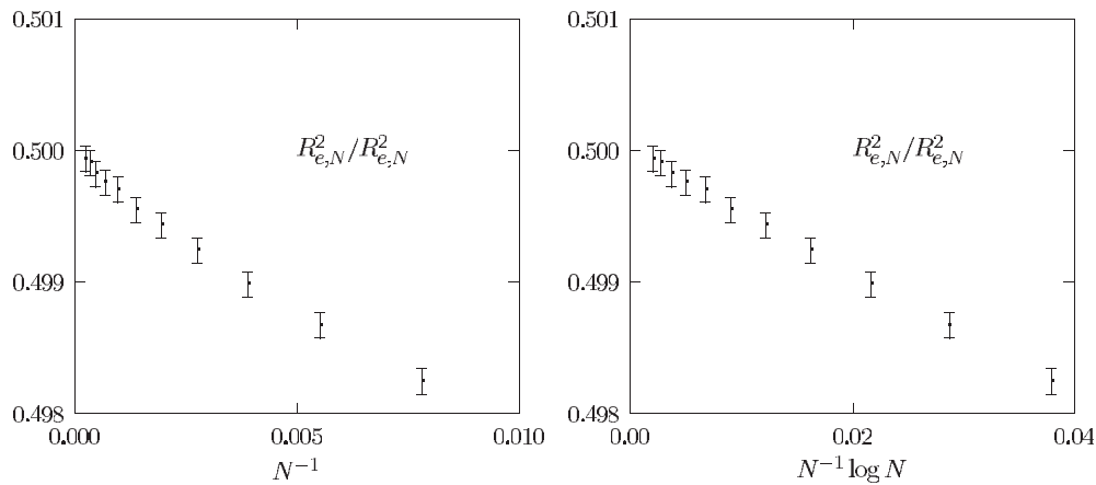
Figure 2. B_N = R_{m,N}^2/R_{e,N}^2 versus N^{-1} and versus N^{-1} \log N for d = 6 , showing the possible presence of a confluent logarithm for the N^{-1} -correction to scaling. We extrapolate B_\infty = 0.5000(2) .
